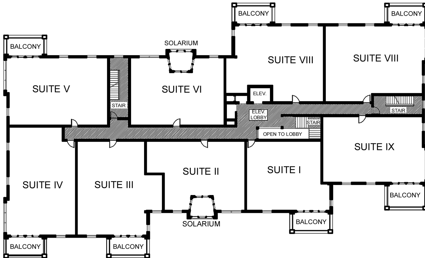
SECOND FLOOR KEY PLAN AVONLEE CONDOMINIUM, PERTH, ONTARIO
